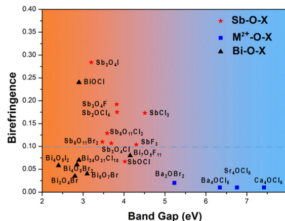
Fig. 5 Comparison between the compounds synthesized in this work ( \star ) and the reported ones in terms of birefringence and bandgap.
