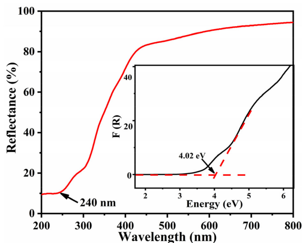
Fig. 4 UV-vis-NIR diffuse reflectance spectrum of 1 .
