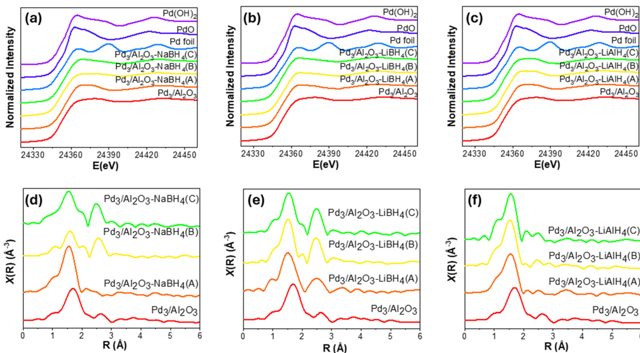
Fig. 1 Pd K-edge XANES spectra of the Pd 3 /Al 2 O 3 activated via treatment with different amounts of (a) NaBH 4 , (b) LiBH 4 and (c) LiAlH 4 along with some standards. Pd K-edge Fourier transformed EXAFS spectra in R -space for Pd 3 /Al 2 O 3 activated via treatment with different amounts of (d) NaBH 4 , (e) LiBH 4 and (f) LiAlH 4 . All EXAFS spectra are shown without phase shift corrections.
