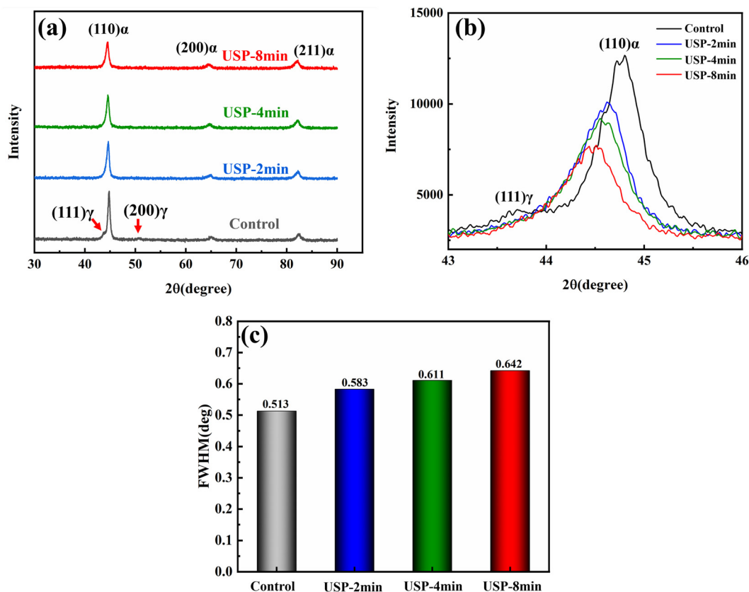
Fig. 8 (a) XRD measurements of the AR-GCr15 bearing steel and the USPed GCr15 steel with peening durations of 2 min, 4 min and 8 min; (b) magnified illustration of the (110) \alpha and (111) \gamma phase peaks; and (c) the full width at half maximum (FWHM) of the \alpha(110) peak for the samples.
