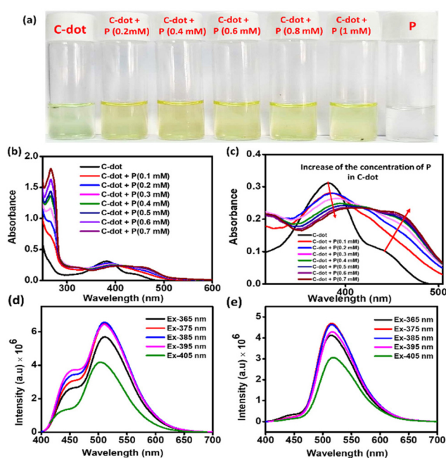
Fig. 2 (a) Photographs of an aqueous solution of carbon dots, and the colour change of the solution after the gradual addition of P amphiphile. (b) Change in the absorbance spectra of the C-dots with increasing P, (c) zoomed-in version of the change. (d) Excitation-dependent emission of the C-dots (e) in CDTP.
