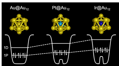
Fig. 1 Schematic illustration of the two-step jellium potential and superatomic orbitals of M@(\text{Au}^+)_n ( M = \text{Au}^+, \text{Pt}^0, \text{Ir}^- ). Reproduced from ref. 95 with permission from the American Chemical Society, Copyright 2020.
