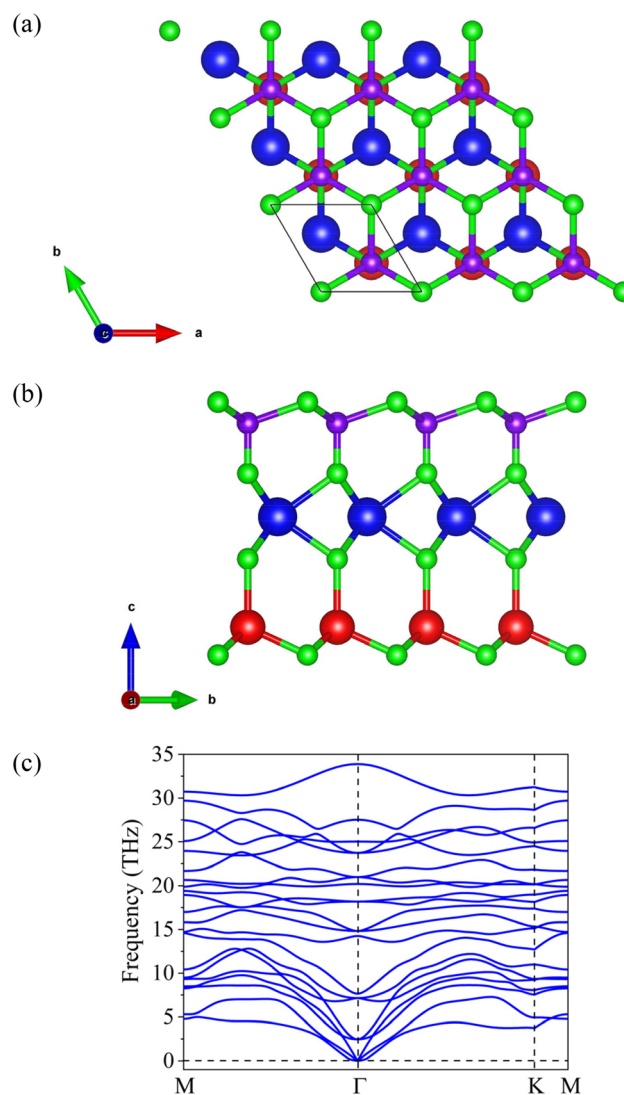
Fig. 1 (a) Top and (b) side views of \text{VGeN}_4 . The green, purple, blue, and red balls denote N, C, V, and Ge elements, respectively. (c) Phonon dispersion of \text{VGeN}_4 .
