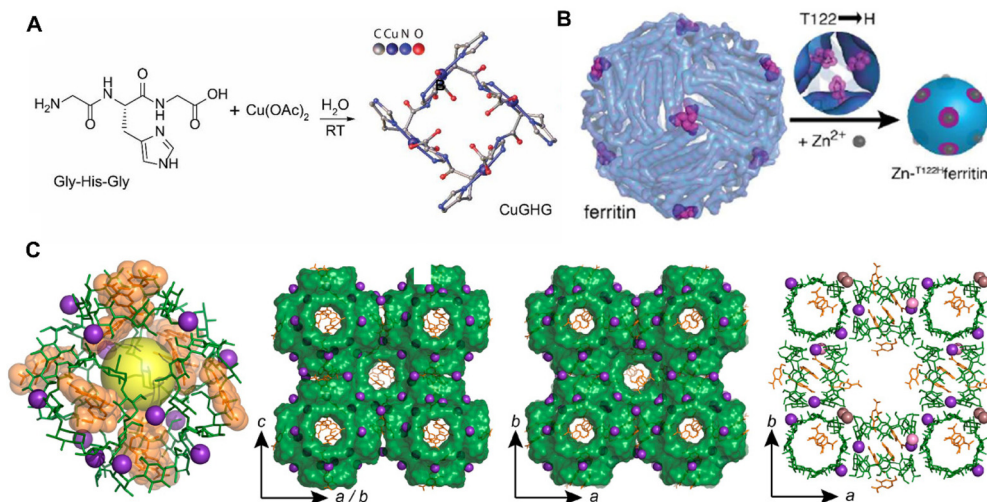
Fig. 4 (A) Synthesis of CuGHG. Reproduced with permission from ref. 63. Copyright 2020 American Chemical Society. (B) Synthesis of \text{Zn}^{\text{T122H}}\text{ferritin} . Reproduced with permission from ref. 64. Copyright 2015 American Chemical Society. (C) Structure of (\gamma\text{-CD})_6 units. Reproduced with permission from ref. 72. Copyright 2020 American Chemical Society.
