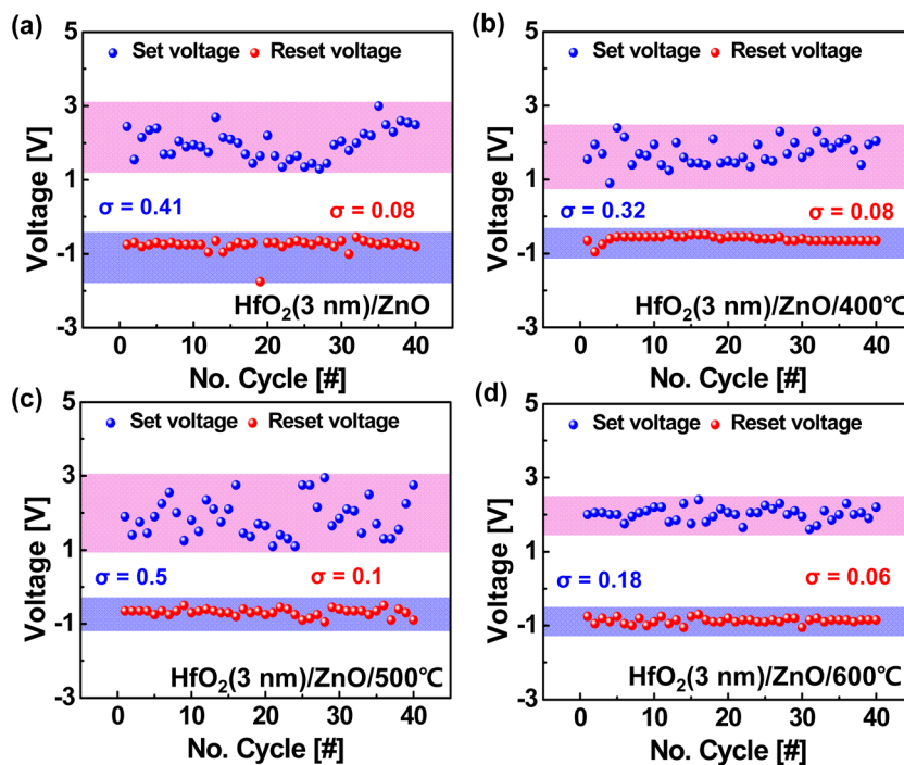
Fig. 6 Obtained VSET and VRESET distributions for 40 consecutive I – V sweeps for bilayer \text{HfO}_2/\text{ZnO} synaptic devices (a) without and with thermal annealing at (b) 400^\circ\text{C} , (c) 500^\circ\text{C} , and (d) 600^\circ\text{C} .
