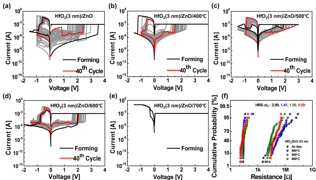
Fig. 5 Typical current–voltage ( I – V ) resistive switching behavior of bilayer \text{HfO}_2/\text{ZnO} synaptic devices (a) without and with thermal annealing at (b) 400^\circ\text{C} , (c) 500^\circ\text{C} , (d) 600^\circ\text{C} , and (e) 700^\circ\text{C} for 1 h in a \text{N}_2 ambient. (f) Distribution and cumulative probability of the high-resistance state (HRS) and low-resistance state (LRS) in 40 consecutive I – V sweeps for bilayer \text{HfO}_2/\text{ZnO} synaptic devices without and with thermal annealing, where the HRS and LRS were extracted at a read voltage of \pm 0.3 \text{ V} .
