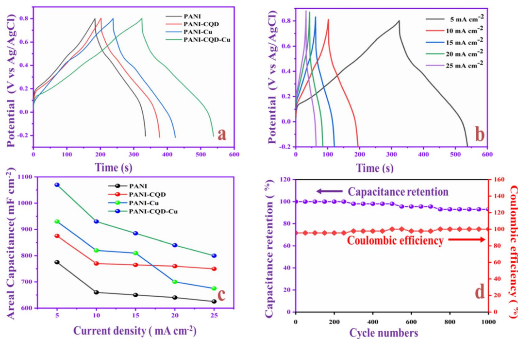
Fig. 12 (a) GCD study of polymer electrodes. (b) Different current density study of the PANI-CQD-Cu electrode material. (c) Specific capacitance of polymer electrodes at different current densities. (d) Cycling stability and coulombic efficiency studies of the PANI-CQD-Cu electrode (circular point: capacitance retention; diamond point: coulombic efficiency).
