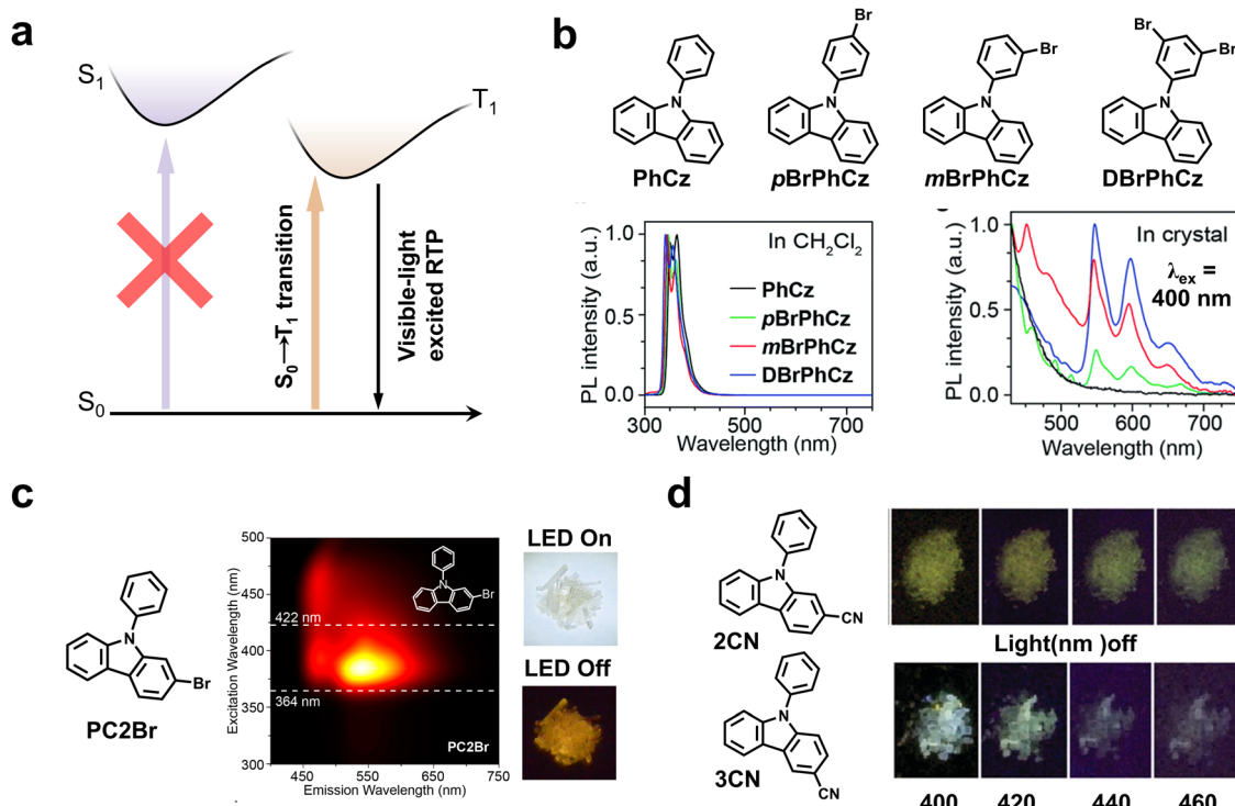
Fig. 7 (a) Simplified Jablonski diagram for interpreting the direct population of T_1 through S_0 \rightarrow T_1 transition. (b) The utilization of the heavy-atom effect for realizing RTP under excitation at 400 nm. Reproduced with permission from ref. 54. Copyright 2019, Royal Society of Chemistry. (c) The LED excitable RTP using Br-substituted aromatic molecules as phosphors based on direct S_0 \rightarrow T_1 transition. Reproduced with permission from ref. 55. Copyright 2024, The author(s). (d) RTP emission of CN-substituted carbazole derivatives under excitation at different visible lights. Reproduced with permission from ref. 56. Copyright 2019, Royal Society of Chemistry.
