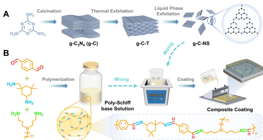
Scheme 1 Schematic illustrating the preparation process of the g-C-NS/poly-Schiff base composite coating. (A) Preparation process of g-C, g-C-T, and g-C-NS. (B) Preparation of poly-Schiff base solution and g-C-NS/poly-Schiff base composite coating.
