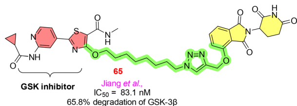
Fig. 18 GSK-3β-PROTACs molecules.
