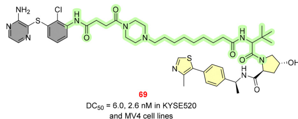
Fig. 20 Nrf2-targeted PROTACs.
