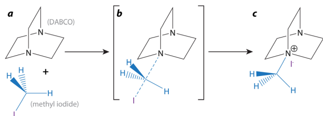
Fig. 13 The reaction of CH 3 I with DABCO showing (a) the initial forms of each, (b) the intermediate bonding environment, and (c) the final form. 176 This figure was reprinted with permission from Aneheim et al. 176 Copyright 2018 Elsevier.
