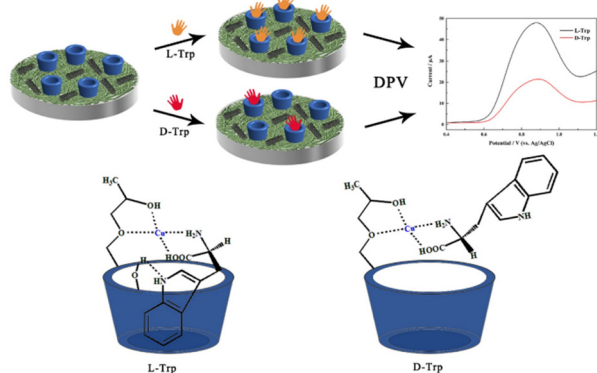
Fig. 7 Schematic representation of electrochemical chiral recognition of tryptophan isomers (reprinted from ref. 81 with permission from Elsevier).
