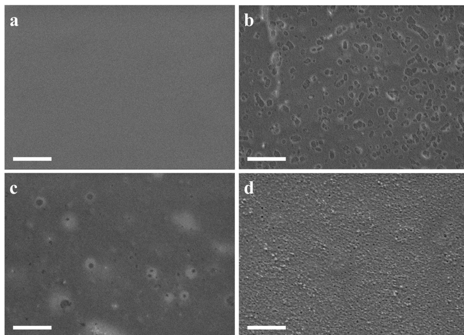
Fig. 1 SEM images of the membrane: (a) HT; (b) PDMS/HT 5 : 50; (c) PDMS/HT 10 : 50; (d) PDMS/HT 20 : 50. Scale bar: 1 \mu\text{m} , accelerating voltage: 2 keV.
