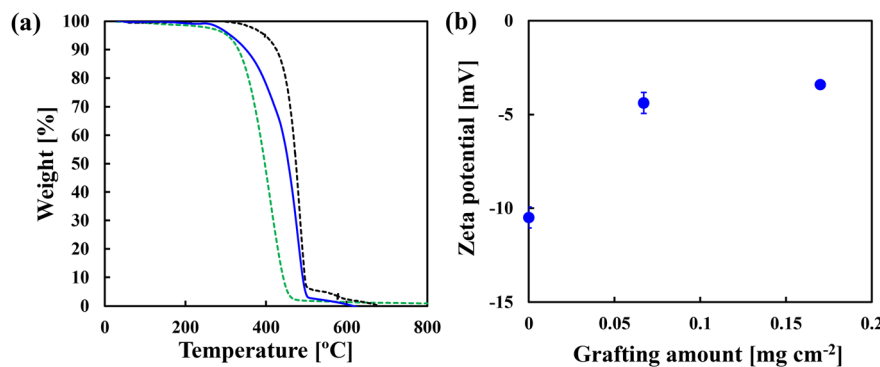
Fig. 2 (a) Thermogravimetric curves of the unmodified polyethylene substrate (black, dashed), PMA (green, dashed) and grafted membrane (blue, solid). (b) Relationship between the grafting amount and the zeta potential of the membrane surface.
