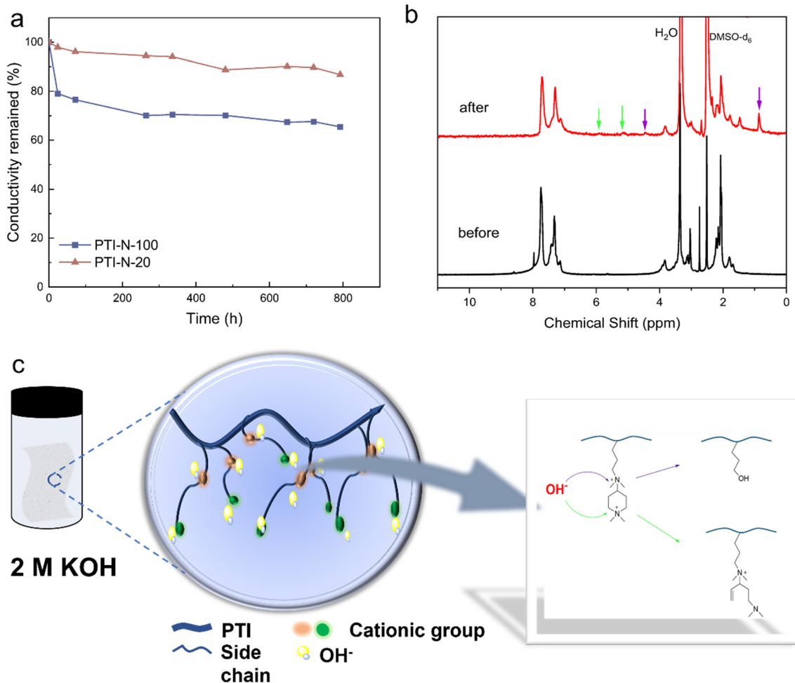
Fig. 8 (a) Curves of ionic conductivity retention versus immersion time of the membranes in 2 M KOH at 80 °C; (b) ^1\text{H} NMR of PTI-N-100 membranes after alkali stability testing and (c) schematic diagram of degradation mechanism.
