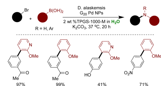
Scheme 35 (A) Ligand-free Pd NPs for biaryl ketone formation in aqueous micellar environment; (B) biogenic Pd(0) NPs in ligand-free Suzuki–Miyaura couplings.
