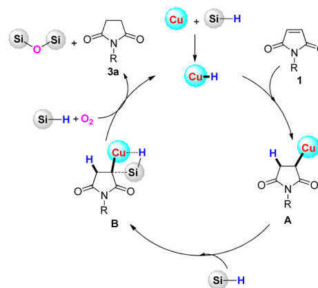
Scheme 3 Proposed mechanism for the \text{Cu(OTf)}_2\text{@CAC} -catalyzed selective reduction of maleimides.
