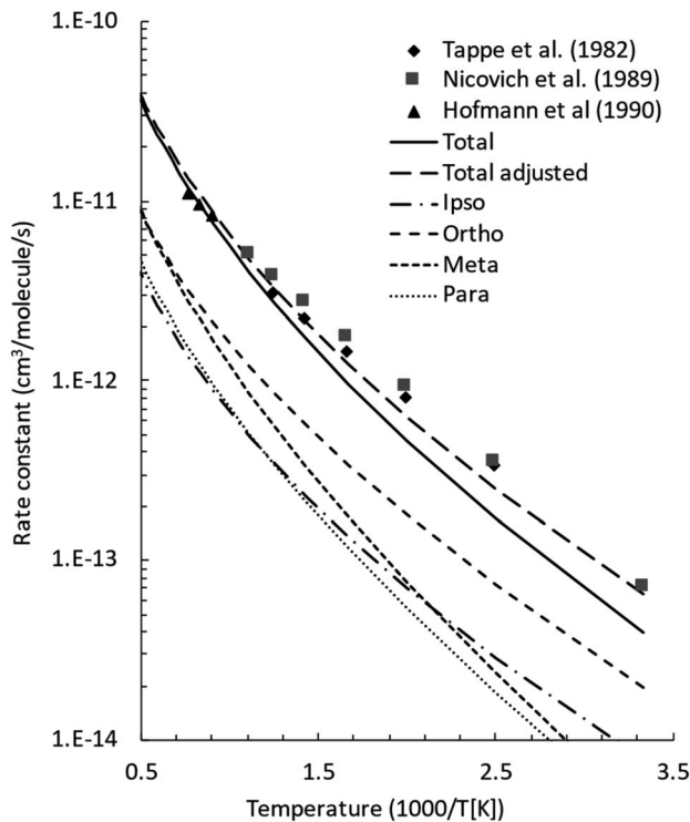
Fig. 6 Comparison between calculated (lines) and experimental (points) rate constants for O( 3 P) addition to toluene. The total adjusted rate was determined by decreasing the energy barrier for all addition channels by 1.2 kJ mol -1 , which is well within the uncertainty of the adopted theoretical model. Symbols: experimental rate constants from Tappe et al. , 24 Nicovich et al. , 23 and Hoffmann et al. 25
