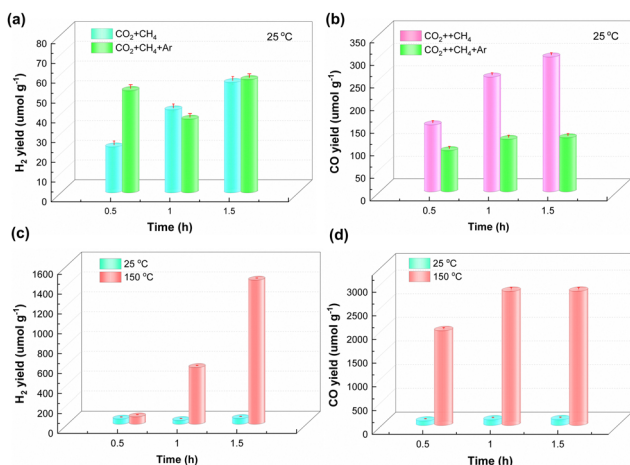
Fig. 7 Performance of NFTC-10 in photocatalytic methane reforming.
