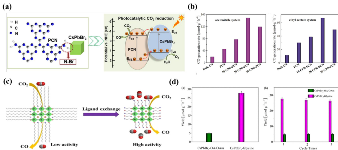
Fig. 13 (a) CsPbBr 3 QDs were anchored on the polymer semiconductor g-C 3 N 4 porous nanosheets via strong N-Br bonds. 111 (b) Generation of CO in the acetonitrile/water (left) and ethyl acetate/water system (right) over various photocatalysts. 111 (c) Glycine-functionalized CsPbBr 3 nanocrystals are constructed through a facile ligand-exchange strategy. 112 (d) Yields of CO generated from CO 2 reduction with CsPbBr 3 -OA/OAm and CsPbBr 3 -glycine NCs as photocatalysts, under Xe-lamp irradiation for 4 h with a 400 nm filter and a light intensity of 100 mW cm -2 (left) and yields of CO generated from CO 2 reduction for three consecutive cycles of 4 h each with CsPbBr 3 -OA/OAm and CsPbBr 3 -glycine NCs as photocatalysts (right). 112
