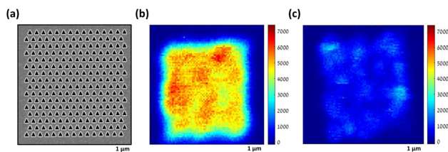
Fig. 5 Second harmonic generation (SHG) intensity maps of our plasmonic device. (a) A typical plasmonic array that was used in this study. (b) SHG scanning of (a), showing that the nonlinear responses are high, yet not uniform, in agreement with the Raman mapping. (c) An example of SHG mapping of plasmonic device in which the milling process was not good (see S5†). Laser power = 2 mW, \lambda_{\text{exc}} = 940 nm.
