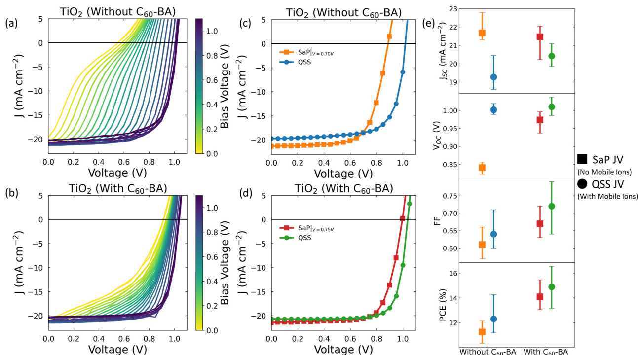
Fig. 2 Stabilise and Pulse measurement for the devices (a) without and (b) with C 60 -BA. The quasi-steady state (QSS) JV s and Stabilise and Pulse (SaP) JV s evaluated at V \approx V_{\text{flat}} for the TiO 2 devices (c) without and (d) with C 60 -BA. (e) Summary of the JV parameters extracted from the SaP JV s and QSS JV s for all measured devices. Error bars indicate the range of measured values.
