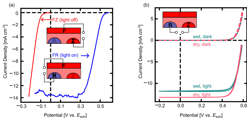
Fig. 4 Photoelectrochemical, electrochemical, and electrical characterization of the three-operating modes of 3T n-lBC Si in both the light and in the dark. (a) Illuminated FR mode CV and dark FZ mode CV vs. E_{\text{soln}} immersed in MV^{2+/+} solution. (b) Illuminated and dark RZ mode CVs for an electrode measured in air (dry) and in MV^{2+/+} electrolyte (wet, E_{\text{soln}} = -0.5 V vs. Ag/AgCl). All illuminated data measured under simulated AM1.5G spectra. Insets show schematics of the contacts used for FR, FZ and RZ measurements.
