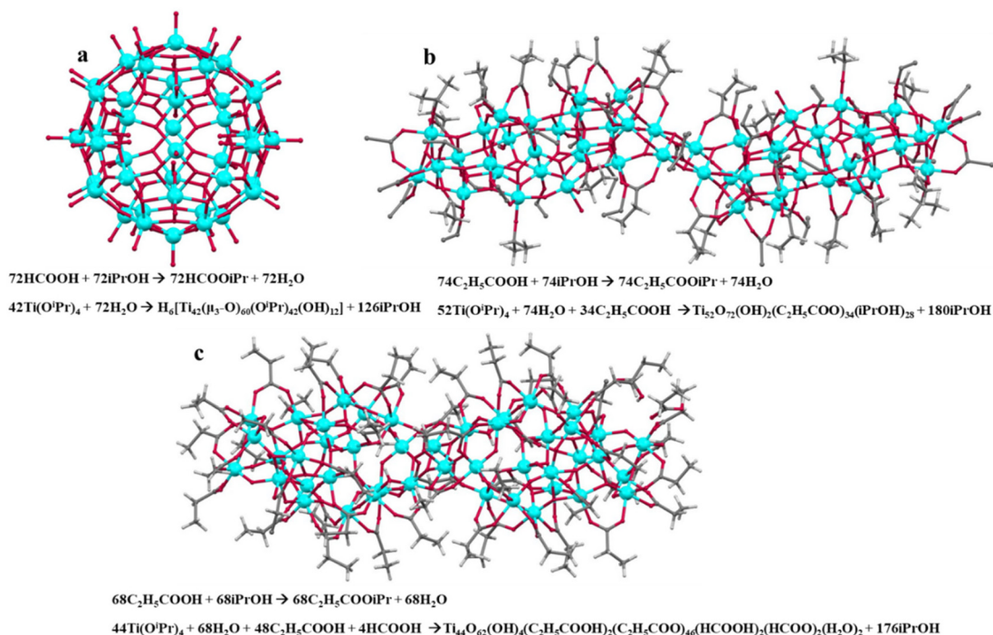
Fig. 4 Overview of the synthesis and structures of (a) \text{Ti}_{42} , (b) \text{Ti}_{52} , and (c) \text{Ti}_{44} -oxo clusters utilizing carboxylates as hydrolysis delayed ligands (a proposed reaction process is depicted). This figure has been adapted/reproduced from ref. 32 with permission from American Chemical Society, copyright 2022.
