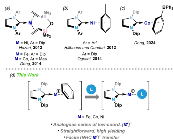
Fig. 1 Key reported examples of (a) (dtvms)-complexes of NHC- M^0 moieties, (b) simple arene complexes of NHC- \text{Ni}^0 moieties, and (c) a cationic arene complex of \text{Co}^I ; (d) this work, demonstrating the facile access to arene adducts of cationic [\text{NHC}\cdot M]^+ moieties, and their utility in [\text{NHC}\cdot M]^+ group transfer.
