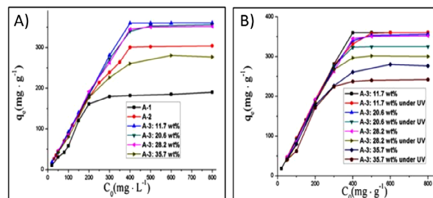
Fig. 2 Adsorption isotherms of uranium ion on Zn-MOF-74 (A) m_{\text{adsorbent}} = 10 mg, pH = 4, t = 5 h and T = 298 K (B) under ambient or after UV (320 nm) irradiation. m_{\text{adsorbent}} = 10 mg, pH = 4, t = 5 h and T = 298 K, t_{\text{irradiation}} = 30 min. Reproduced with permission from Journal.
