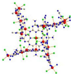
Fig. 2 Section of the structure showing the tilted connectivity pattern between one (\text{C}_{12}\text{N}_{20}\text{H}_8)^{4-} unit with four adjacent ones via \text{-N-In-N-} bonding.
