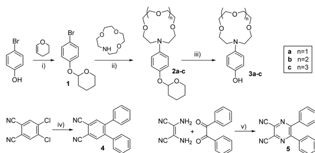
Scheme 1 Synthesis of ligands and precursors – (i) pyridinium 4-toluenesulfonate, anhydrous dichloromethane, argon, room temperature, 2 h, 98%; (ii) Pd 2 (dba) 3 , NaOtBu, Dave Phos, anhydr. toluene, argon, 80 °C, 12 h, 80–92%; (iii) 4-toluenesulfonic acid, methanol, argon atmosphere, room temperature, 2 h, 75–90%; (iv) phenylboronic acid, PdCl 2 (PPh 3 ) 2 , NaBr, saturated K 2 CO 3 , dioxane, argon, reflux, 6 h, 78%; (v) acetic acid, reflux, 2 h, 75%.
