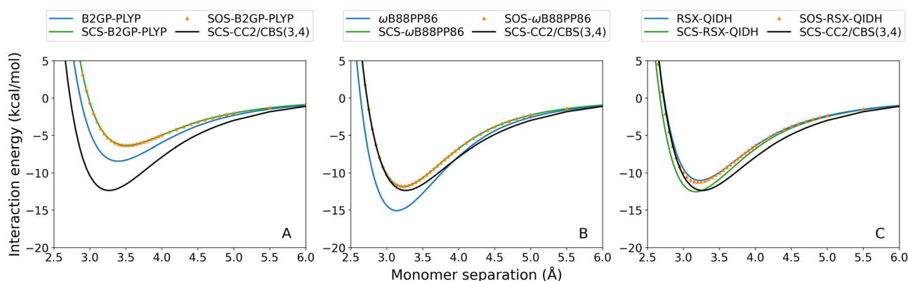
Fig. 8 Toluene-TCNE 3A' dissociation curves for representative TD-DHDFAs and their SCS/SOS variants: (A) B2GP-PLYP; (B) \omega B88PP86; (C) RSX-QIDH.
