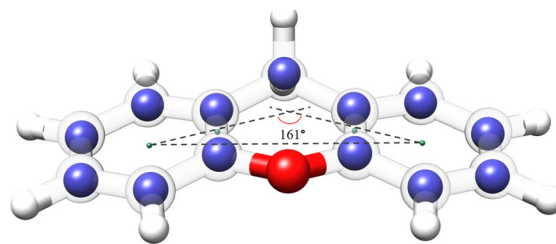
Fig. 6 Overlay between the r_s and the r_e structures for the xanthenes monomer calculated at the B3LYP-D3BJ/def2-TZVP level of theory. The blue spheres represent the carbon positions determined using the Kraitchman's equations ( r_s ), whereas the semi-transparent structure represents the theoretical structure ( r_e ) of xanthenes. Rendered using UCSF ChimeraX software. 16
