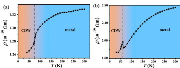
Fig. 4 Temperature dependence of theoretical resistivity for 2H-TaS 2 . (a) Bulk samples, (b) mono-layer samples.
