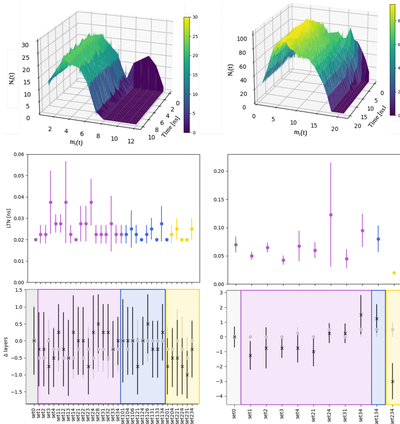
Fig. 3 Left column refers to Au 55 h -Pd 55 h and right column to Au 561 h -Pd 561 h . Top: Distribution of the number of atoms per layer with \rho_{\text{Au}} = 0.5 , \rho_{\text{Pd}} = 1.5 , \eta_{\text{Au}} = 0.02 eV and \eta_{\text{Pd}} = 0.8 eV, aka set 34. The colour gradient represents N_i(t) . Middle: Mean value of the LTN and its standard deviation over independent simulations for each MEI. Vacuum, labelled as set0, is in grey. Bottom: Difference between the number of layers N_i(t) in an MEI and the vacuum ( \Delta layers) averaged over the independent simulations and their standard deviation at the initial time (grey full circles) and after 10 ns for Au 55 h -Pd 55 h and 20 ns for Au 561 h -Pd 561 h (black stars). For the middle and bottom rows, the x-axis labels the environment; MEIs are coloured in accordance with chemical species interactions: only Pd is blue (MEI-P); only Au is yellow (MEI-A); both Au and Pd interacting (MEI-AP) are violet. For a full description of the MEI, see Table S1 of the ESI.†
