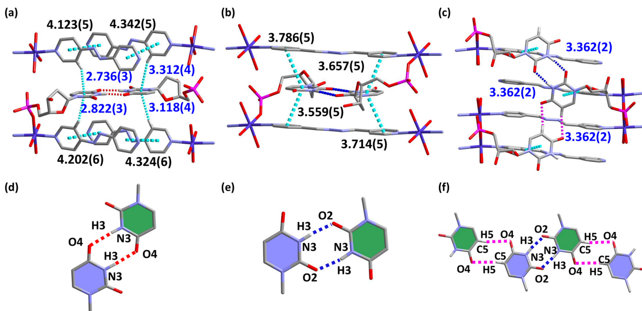
Fig. 2 The hydrophobic chemical environment formed by the auxiliary ligand in (a) 2 , (b) 3 , and (c) 5 , in which nucleobases were fixed by \pi - \pi stacking interaction. The formed U-motifs III and IV in (d) 2 and (e) 3 respectively. The U-motifs I (pink dashed line) and IV (dark blue dashed line) formed in (f) 5 .
