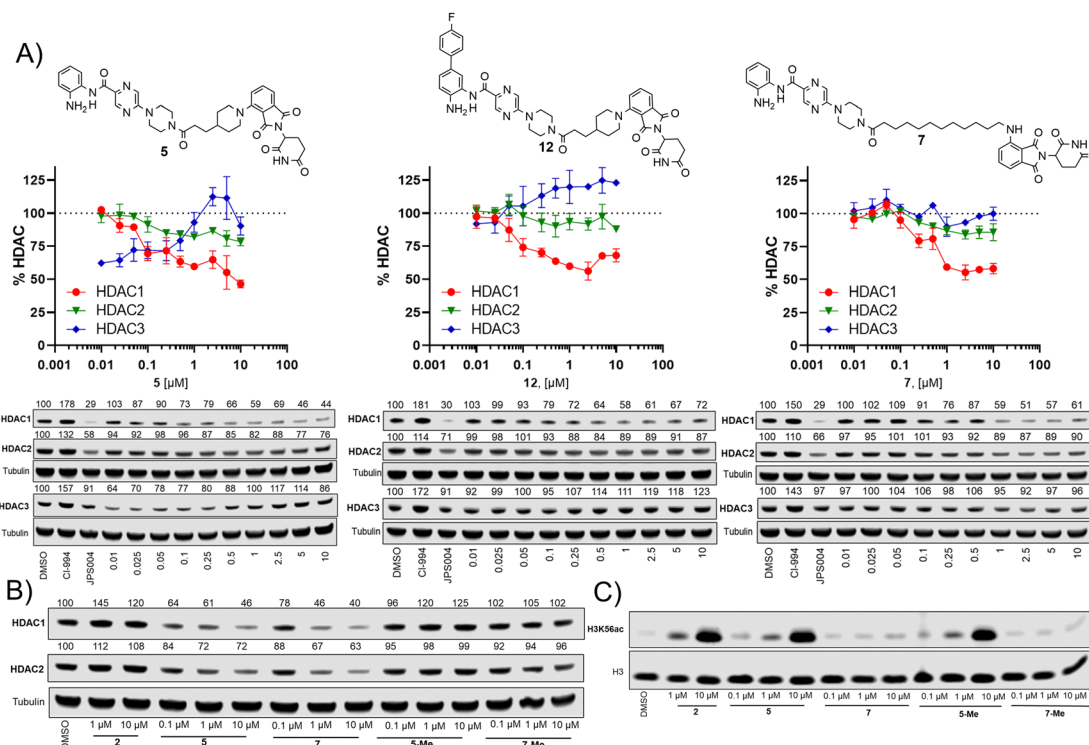
Fig. 4 (A) Dose response degradation of HDAC1, HDAC2, HDAC3 in the presence of 5 , 7 and 12 in HCT116 cells after 24 h. HDAC1, HDAC2, HDAC3 abundance were determined by quantitative western blotting with antibodies for HDAC1, HDAC2, HDAC3. Error bars represent the variation between two independent biological replicates. (B) HDAC1 and HDAC2 degradation is compromised in the presence of 5-Me and 7-Me that do not bind the cereblon E3-ligase. (C) H3K56 acetylation levels were determined in the presence of 2 , 5 , 7 , 5-Me and 7-Me by quantitative western blotting with an antibody for H3K56ac.
