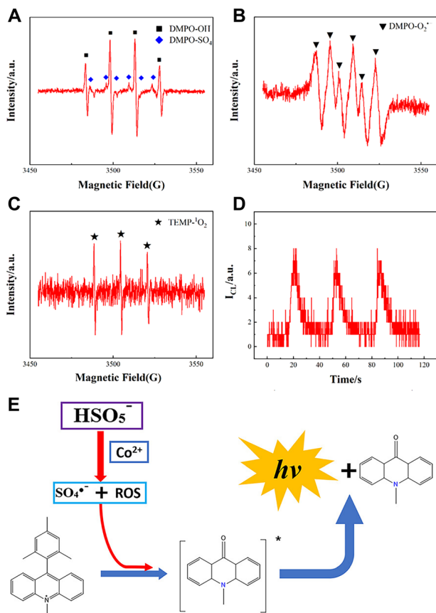
Fig. 8 ESR spectra of (A) OH • /SO 4 •- , (B) O 2 •- and (C) 1 O 2 in the Acr + -Mes/KHSO 5 system. (D) CL intensity of the Acr + -Mes/H 2 O 2 system. (E) CL mechanism of the Acr + -Mes/KHSO 5 system and the detection of Co 2+ . [Acr + -Mes]: 0.1 mM; [KHSO 5 ]: 2 mM; [H 2 O 2 ]: 2 mM; [PBS]: 0.1 M, pH = 7.0. PMT voltage: -900 V. Reprinted with permission from ref. 15, Copyright 2023 American Chemical Society.
