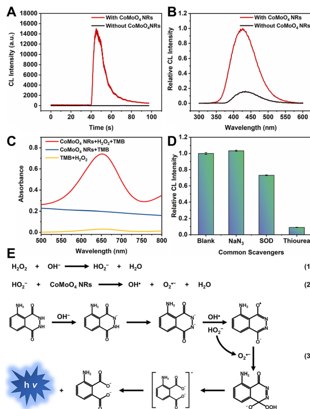
Fig. 9 (A) CL intensity-time curves and (B) CL spectra of the luminol/H 2 O 2 system in the absence and presence of CoMoO 4 NRs. CBS pH 11.0, [luminol]: 1 μM; [H 2 O 2 ]: 50 μM; [CoMoO 4 NRs]: 20 μg mL -1 . (C) UV-vis absorption spectra of TMB/H 2 O 2 , CoMoO 4 NRs/H 2 O 2 , and CoMoO 4 NRs/H 2 O 2 /TMB systems. NaAc/HAc buffer solution pH 4.0, [TMB]: 0.1 mM; [H 2 O 2 ]: 25 mM; [CoMoO 4 NRs]: 50 μg mL -1 . (D) Relative CL intensity of luminol/H 2 O 2 /CoMoO 4 NRs with common radical scavengers including 1 mM NaN 3 , 5 μg mL -1 SOD, and 1.0 mM thiourea. CBS pH 11.0; [luminol]: 1 μM; [H 2 O 2 ]: 50 μM; [CoMoO 4 NRs]: 20 μg mL -1 . (E) CL mechanism of the luminol/H 2 O 2 /CoMoO 4 NR system. Reprinted with permission from ref. 61, Copyright 2024 American Chemical Society.
