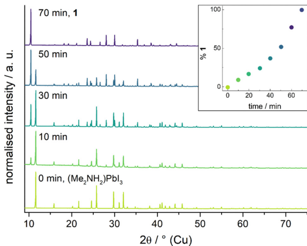
Fig. 1 Diffraction patterns of the powder taken from a suspension of (\text{Me}_2\text{NH}_2)\text{PbI}_3 in acetone. Percentage of 1 in the mixture as determined by Rietveld refinement shown as an inset.
