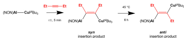
Scheme 8 Experimental insertion of internal 3-hexyne in the Cu–Al bond of the [\text{Bu}_3\text{PCuAl}(\text{NON})] complex. 68
