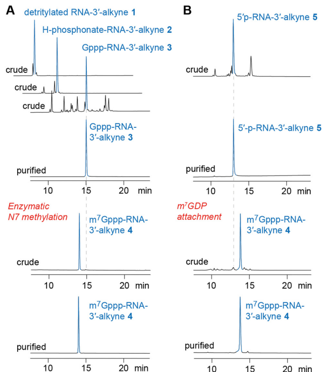
Fig. 3 HPLC analysis of m^7 Gppp-RNA 3'-alkyne preparations (exemplified for m^7 G-5'-ppp-5'-( m_2^6Am )(Am)(Cm)( m^3Um )(3'-O-propargyl-A, RNA 4). (A) Path for chemoenzymatic synthesis. (B) Path for all-chemical synthesis (for details see Fig. 2 and Table 1 and the ESI†).
