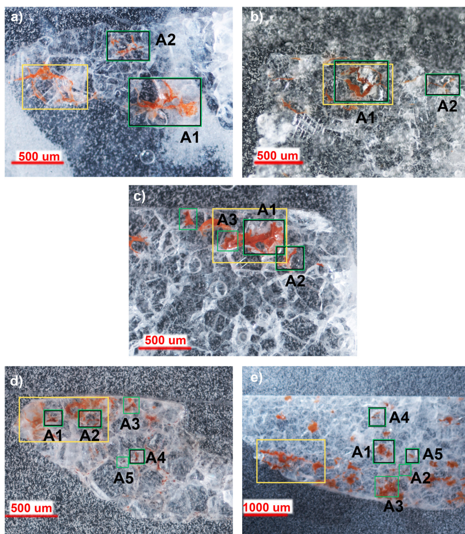
Fig. 2 Optical microscope images (4–10 \times magnification) of the thin sections coming from the Duomo and the Baptistry of Florence (D, L10-C2, L4P10H3) (a, b, c) and from monumental fountains in Villa La Petraia (P1, F1) (d, e). Green squares in all the images, refer to \mu -XRPD and \mu -XRF measurements while black squares refer to \mu -Raman analysed areas. In yellow squares SEM-EDS and FTIR chemical imaging analysed areas.
