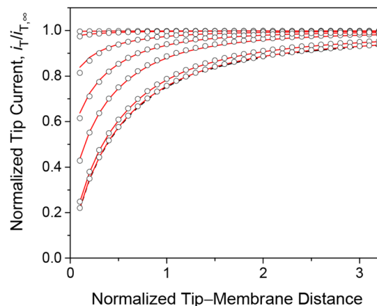
Fig. 3 Steady-state approach curves simulated for two-step (solid lines) and one-step (circles) transport with \kappa = 10 and \rho = 1 , and \lambda ( = 0.3\lambda_{mem} in eqn (25)) = 10^2 , 3 \times 10^{-1} , 1 \times 10^{-1} , 1 \times 10^{-2} , and 1 \times 10^{-3} from the top to the bottom. Black dashed line represents an impermeable membrane.
