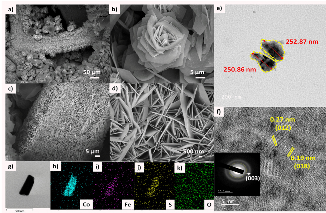
Fig. 2 FESEM images of (a) and (b) \text{S-CoFeLDH/NF} and (c) and (d) \text{CoFeLDH} at different resolutions. (e) TEM image, (f) HR-TEM image with the inset showing the SAED pattern of \text{S-CoFeLDH/NF} and (g)–(k) elemental maps of \text{Co} , \text{Fe} , \text{S} and \text{O} of \text{S-CoFeLDH/NF} .
