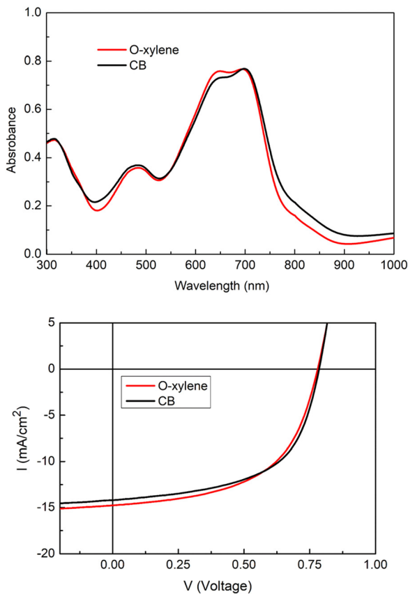
Fig. 3 Absorption spectra and I - V curves of PTB7-Th:AzaTk blend film deposited from o -xylene and chlorobenzene solutions.
