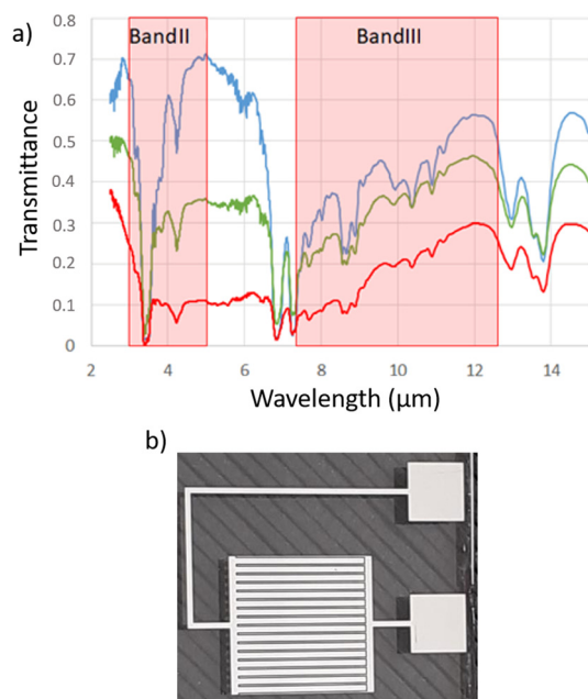
Fig. 5 (a) IR spectrum of Isopar L (blue), NP AZO at 10 \text{ mg mL}^{-1} (green) and 40 \text{ mg mL}^{-1} in Isopar L. (b) Optimized interdigit electrodes with 63% reflective surface and 50 \mu\text{m} gap between electrodes.
