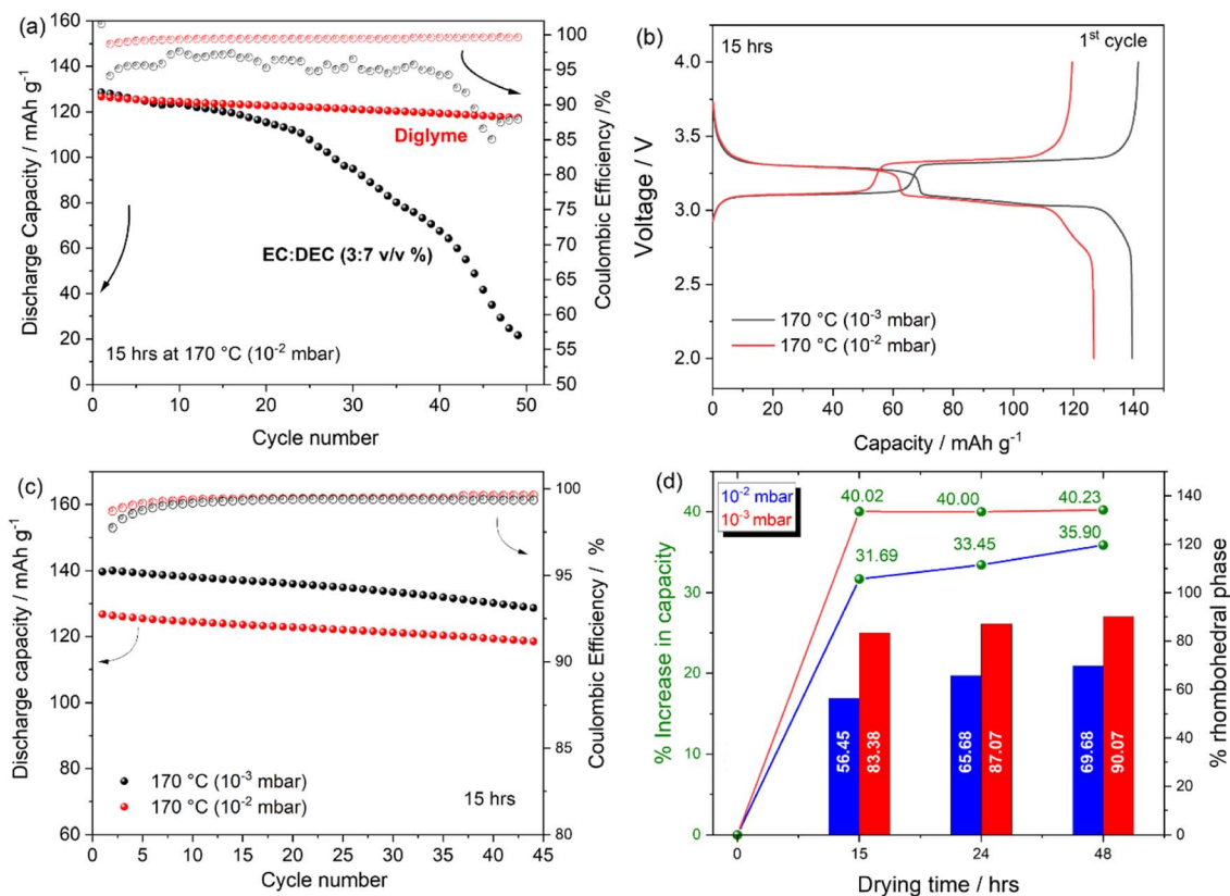
Fig. 8 (a) Cycling behaviour of PW-based electrode dried at 170 °C (10 -2 mbar) in sodium half-cell using 1 M NaPF 6 in EC:DEC (3:7 v/v%) (black curve) and 1 M NaPF 6 in diglyme (red curve). (b) First cycle voltage profiles and (c) corresponding cycling behaviour of PW-based electrodes dried for 15 hours at 170 °C under a dynamic vacuum of 10 -2 mbar (red curve) and 10 -3 mbar (black curve). (d) Comparative data of the percentage increase in capacity relatively to the percentage of rhombohedral phase formed upon dehydration at 170 °C for 15, 24, and 48 hours using a dynamic vacuum of 10 -2 and 10 -3 mbar. Tests are conducted at 25 °C within the 2.0–4.0 V range.
