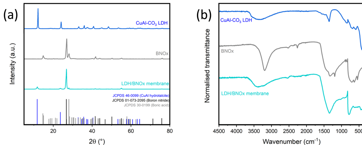
Fig. 1 (a) pXRD patterns and (b) FT-IR spectra of CuAl–CO 3 LDHs (blue), BNOx (grey) and LDH/BNOx nanocomposite (turquoise). pXRD reference patterns are provided for CuAl hydroxalcite, boron nitride and boric acid.
