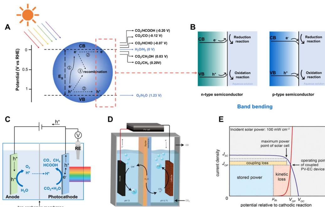
Fig. 1 (A) Schematic of photocatalytic CO 2 reduction, illustrating the three main steps of the process, and (B) band bending of an n-type and p-type semiconductor at the semiconductor/liquid interface. 12 Copyright 2015, Springer Nature. (C) Schematic of a typical photoelectrochemical CO 2 reduction device. (D) Schematic of the PV-EC CO 2 reduction device. 13 Copyright 2017, Springer Nature. (E) General current density-voltage diagram for a coupled PV-EC system. 14 Copyright 2013, Proceedings of the National Academy of Sciences.
