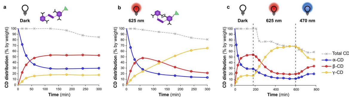
Fig. 5 Distribution of \alpha -, \beta -, and \gamma -CD as function of time for enzymatic reactions starting from \alpha -CD ( 10 \text{ mg mL}^{-1} ) with CGTase ( 65 \mu\text{L mL}^{-1} reaction mixture) in sodium phosphate buffer (100 mM, pH 7.5) in the presence of template ipAzo (10 mM). Reaction conditions: (a) in darkness having primarily the trans isomer, (b) under continuous red light irradiation (625 nm) promoting trans to cis isomerisation and (c) starting in darkness, then under irradiation with red light and finally under irradiation with blue light (470 nm) to promote cis to trans isomerisation.
